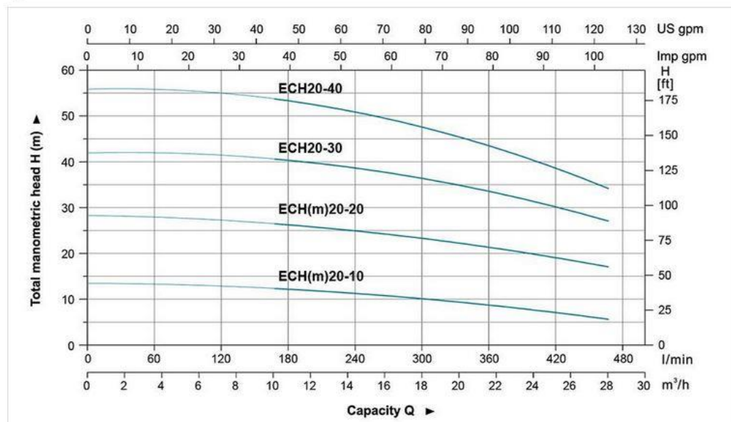
Hydraulic Performance Curves
