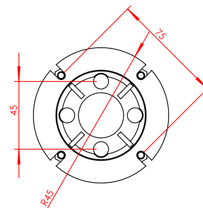
63B14
