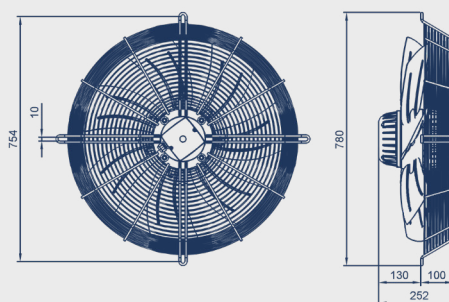
VIK63-G (without frame)
