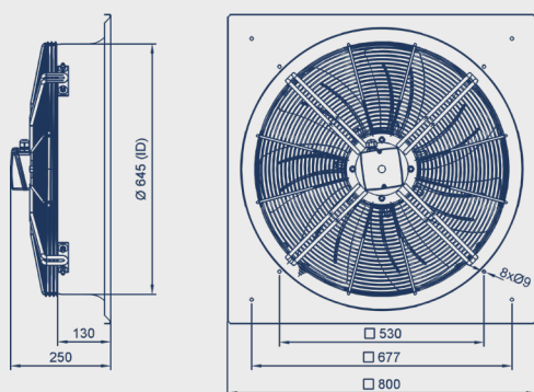
VIK63-R (with frame)
