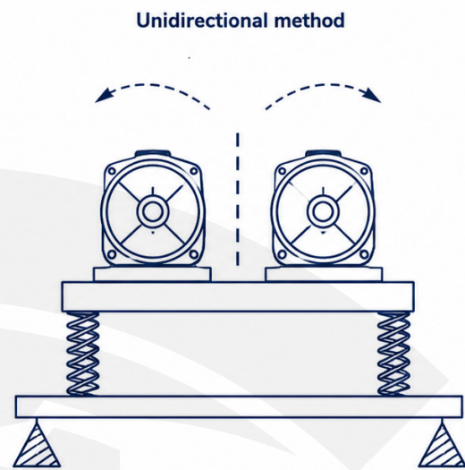
Vibrating force in a single direction, in a counter rotating motor
