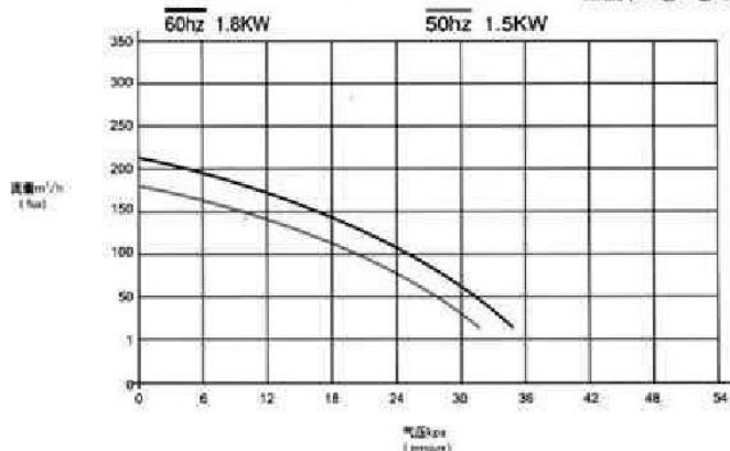
the technology parameter of the HG series vortex gas pump (only for reference,not for test gist)
