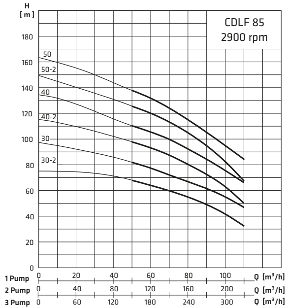
Performance curves are given according to ISO9906: 2012 Gr3B.
